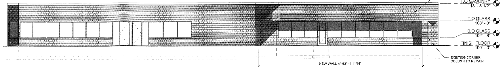
2 EAST ELEVATION 1/8" = 1'-0"
